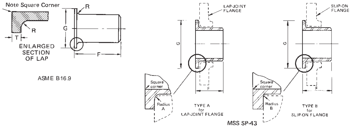
ASME B16.9 MSS SP-43 (mm)
